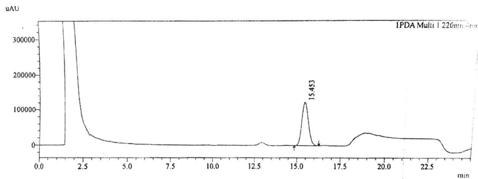
Figure 5 Leuprolide acetate alkali degradation
