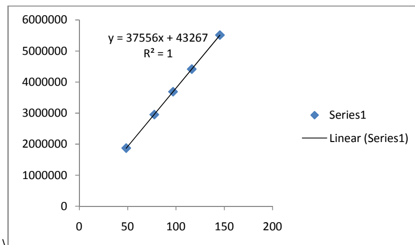
Fig. 3 Calibration curve of Leuprolide acetate
