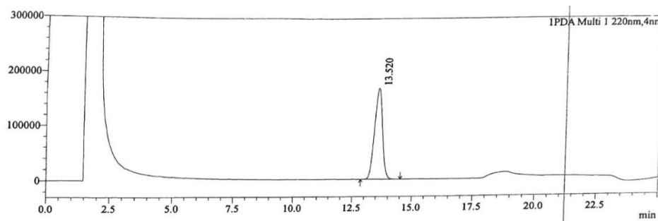
Fig. 2 Chromatogram of leuprolide acetate test sample
