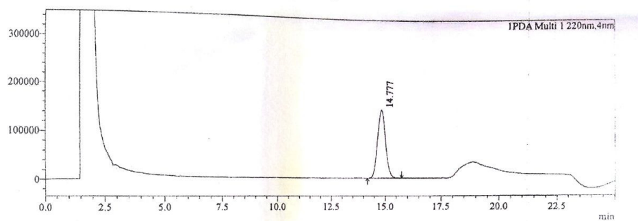
Figure 6 Leuprolide acetate peroxide degradation
