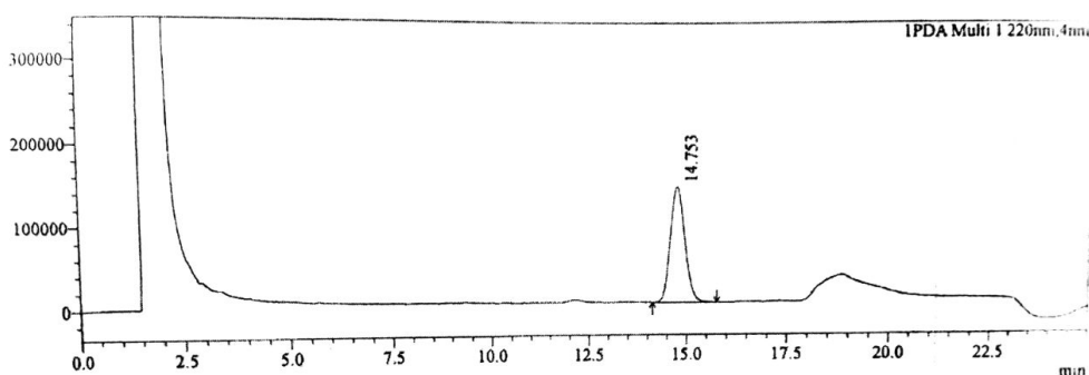
Figure 4 Leuprolide acetate acid degradation
