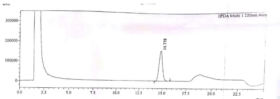
Figure 13 Leuprolide acetate Thermal degradation
