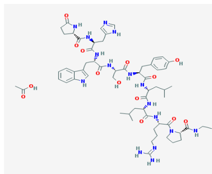
Fig. 1 Leuprolide acetate structure
