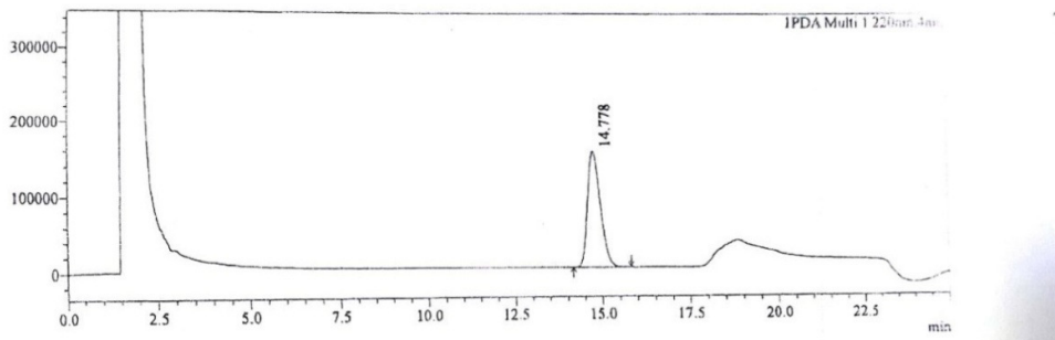
Figure 7 Leuprolide acetate photolytic degradation
